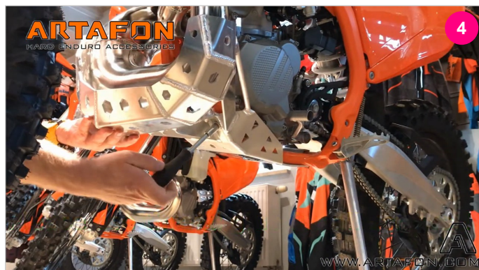
GRAB SCREWS IN THE FRAME SOCKETS USING WASHERS
